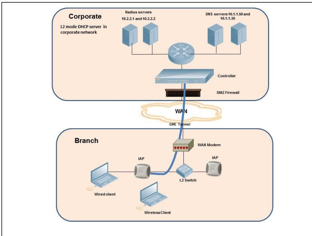
Figure 138 Scenario 4 - GRE: Single Datacenter Deployment with No Redundancy
